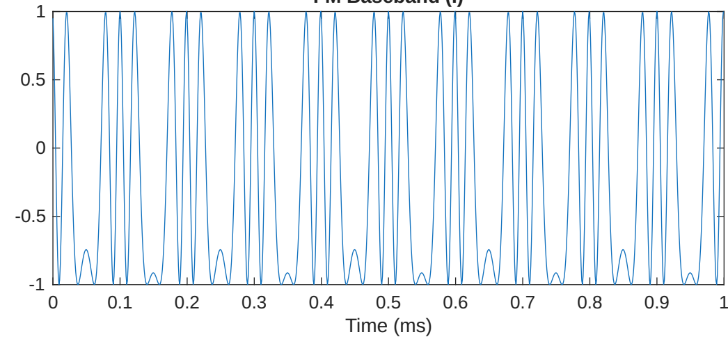
FM Baseband (I)
